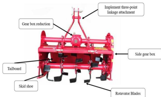
Fig.1: Components of Rotavator [8]
