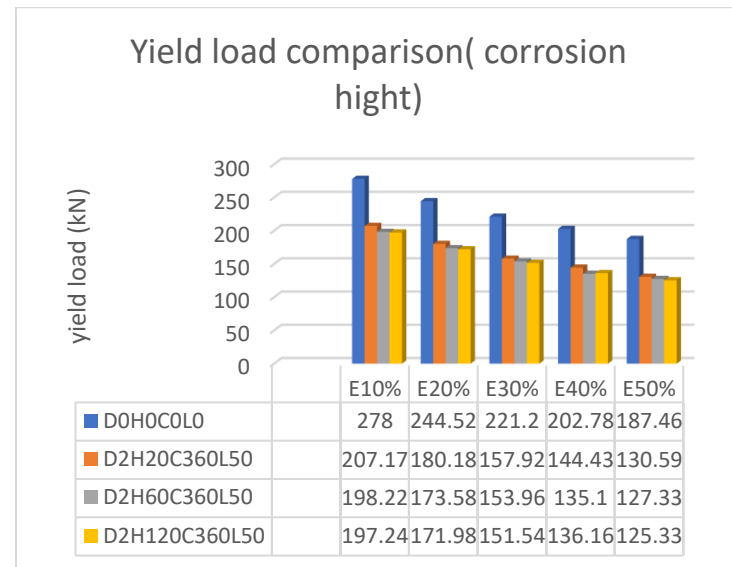
Fig.10. Yield load comparison (corrosion height)
