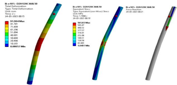
Fig .15. total deformation, stress & force reaction of model D2H120C360L50
