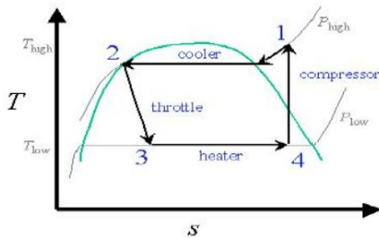
Fig.2. T-S diagram of vapour compression cycle
