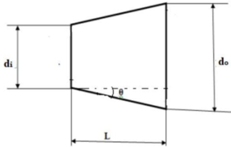
Fig.8. Line diagram of Diffuser
